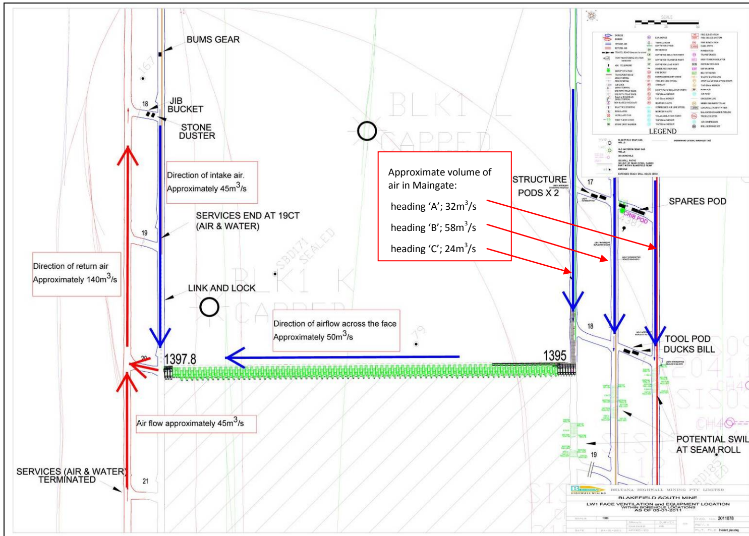
Figure 8: LW1 ventilation diagram
