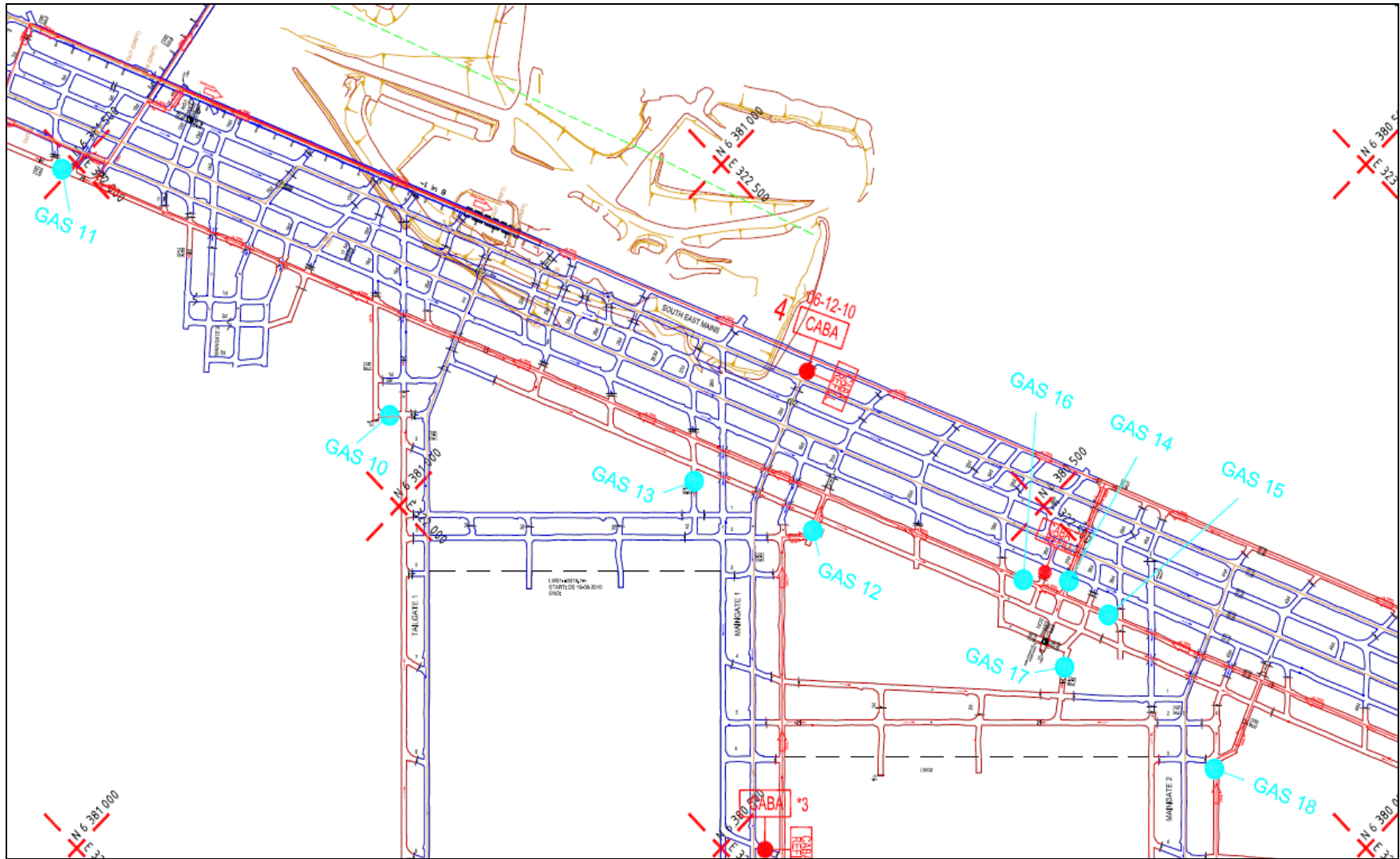
Figure 21: Plan of part of BSM showing mine ventilation and location of gas monitoring sites
