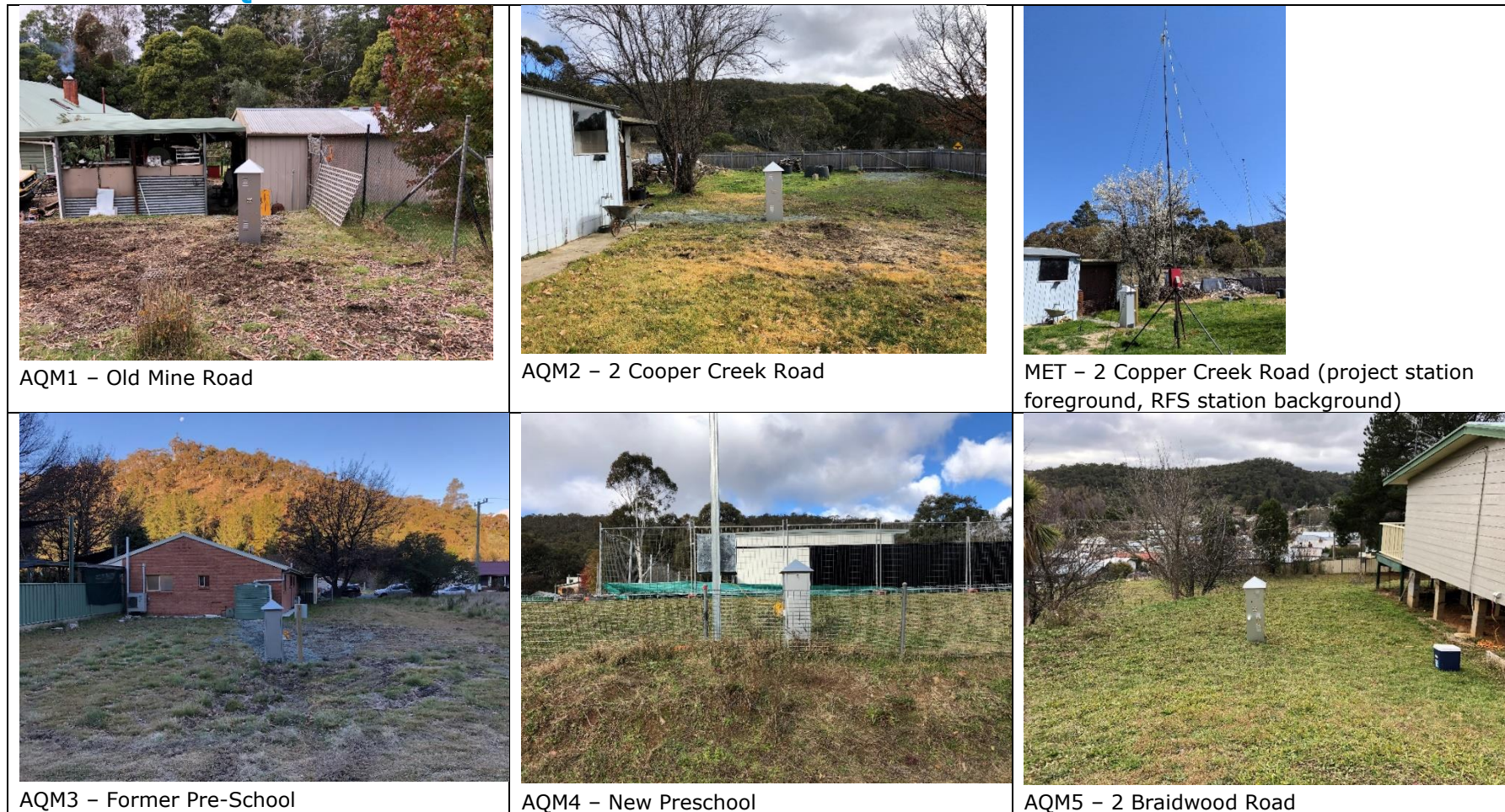
Figure B: High-volume air samplers and meteorological station in-situ in Captains Flat, NSW
