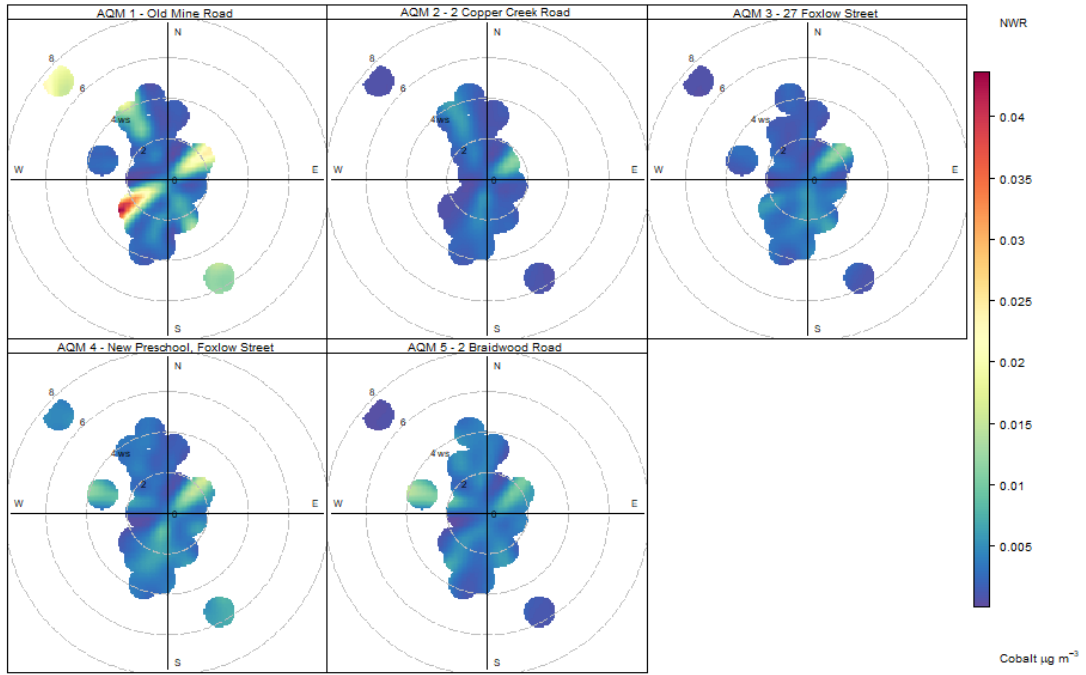
Figure 5-29: Polar plots showing 24-hour cobalt concentration and 24-hour average wind speed and direction at each monitoring location, from 22 June 2021
