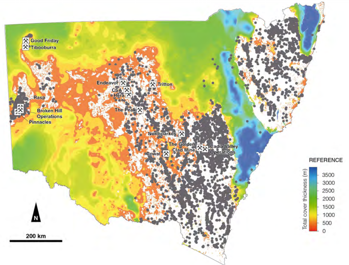
Total cover thickness with metallic mineral occurrences
