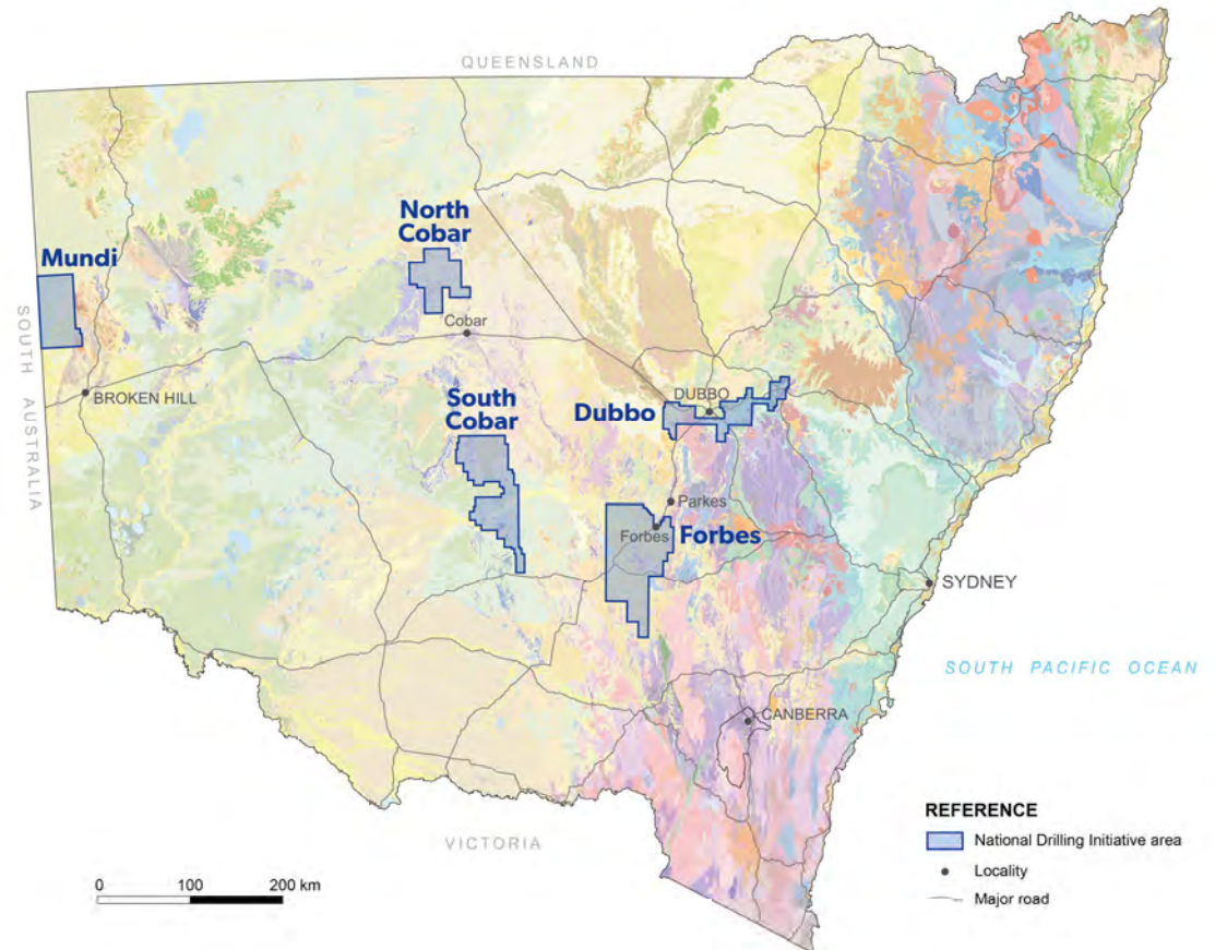
Seamless Geology of NSW v1.1
