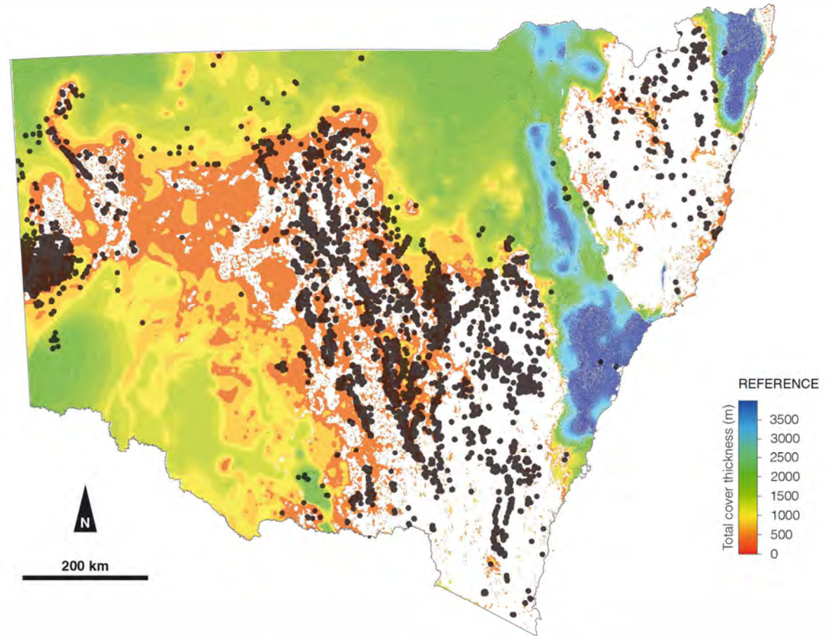
Total cover thickness with metallic mineral drill holes
