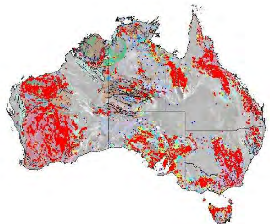
Publicly available drilling data (with exposed basement geology and TMI 1VD)
