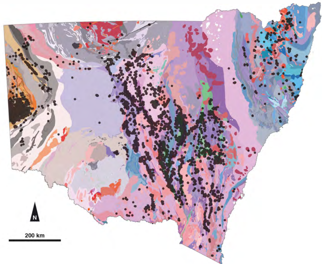
Basement geology with metallic mineral drill holes
