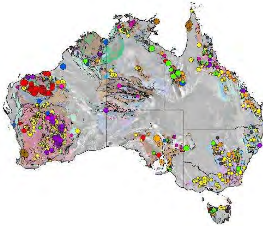
Australia's known mineral deposits (with exposed basement geology and TMI 1VD)
