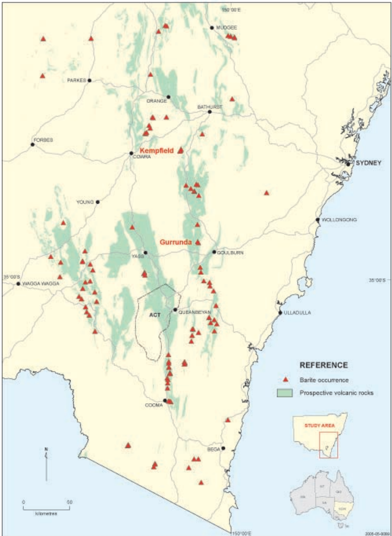
Figure 2. Barite occurrences and prospective rocks, eastern Lachlan Orogen, New South Wales
